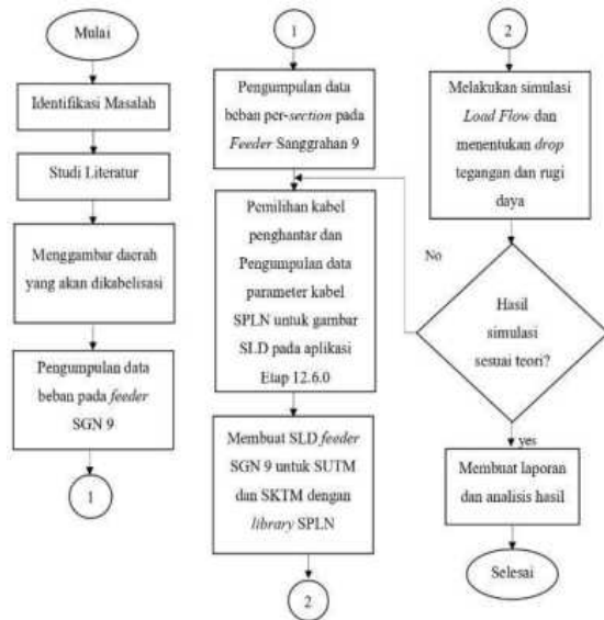
Gambar 1. Flowchart penelitian
